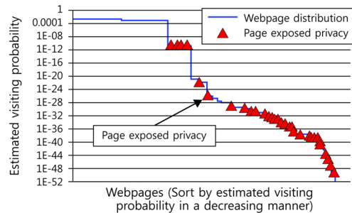
〈Figure 8〉 Distribution of Webpages in Website W2
